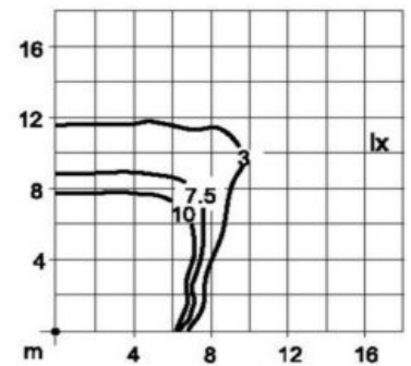
Metropolitan Symmetric 1 x HIT 150 W h= 4m
