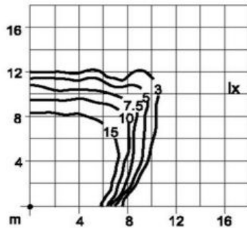
Metropolitan Asymmetric 1 x HIT 150 W h= 4m
