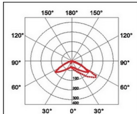
— C0 / C180 - - - - C90 / C270 Cd / 1000 lm \eta_{lm} = 44.5\%
